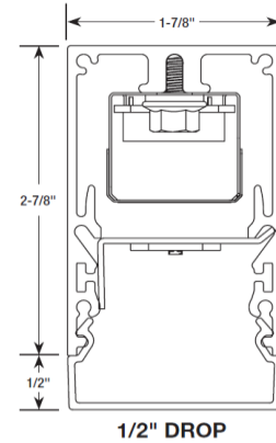
Luminaire Cross Section
